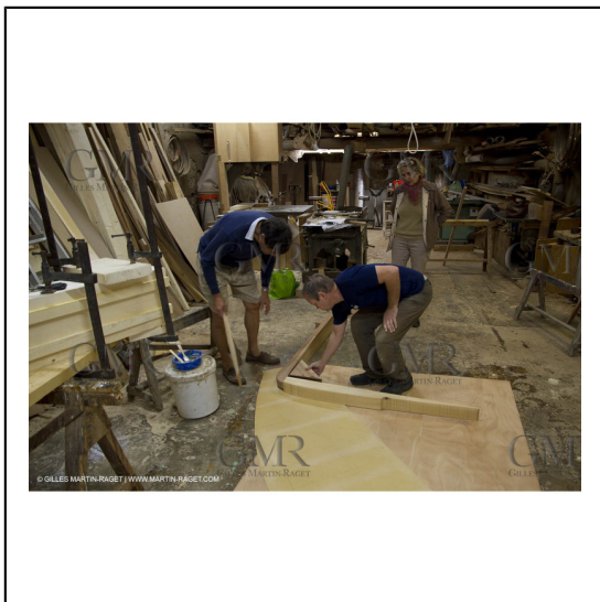
5/11/2011 - Marseille (FRA,13) - Alcyon - construcion - Rendez vous de Marc et Edith Frilet dans l'atelier de Daniel Scotto*** 5/11/2011 - Marseille (FRA,13) - Alcyon - construction - Marc and edith Frilet meet Daniel Scotto in his workshop
