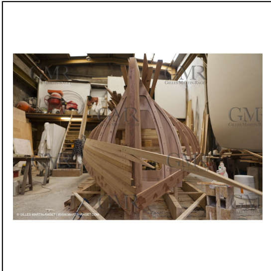
30/01/2012 - Marseille (FRA,13) - Construction d'Alcyon : pose des bordés***30/12/2012 / Marseille (FRA,13) / Alcyon building at boat yard
